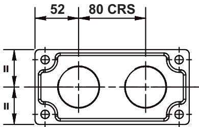
2 mains entry maximum entry size CM50
