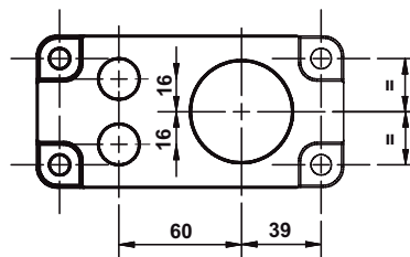
1 main & 2 auxiliaries maximum main entry size CM50 auxiliary entry size CM20
