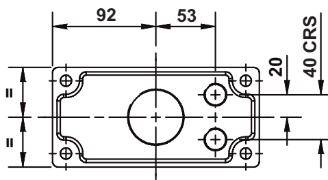
2 mains & 1 auxiliary maximum main entry size CM40 auxiliary entry size CM20
