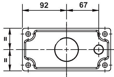
2 mains entry maximum entry size CM50
