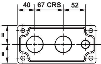
2 mains & 1 auxiliary maximum main entry size CM40 auxiliary entry size CM20
