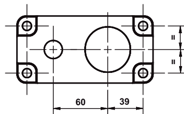
1 main & 1 auxiliary maximum main entry size CM50 auxiliary entry size CM20
