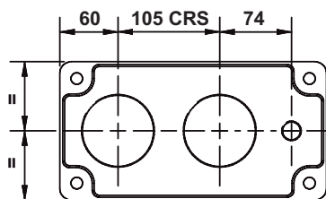
2 mains & 1 auxiliary maximum main entry size CM63 auxiliary entry size CM20
