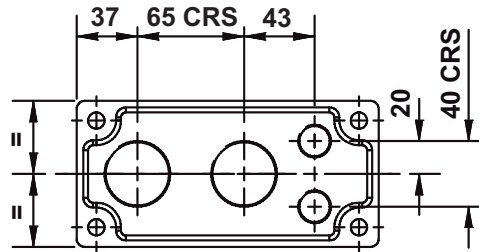
2 mains & 2 auxiliaries maximum main entry size CM40 auxiliary entry size CM20
