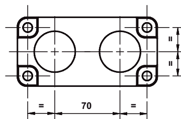
2 main entries maximum entry size CM40
